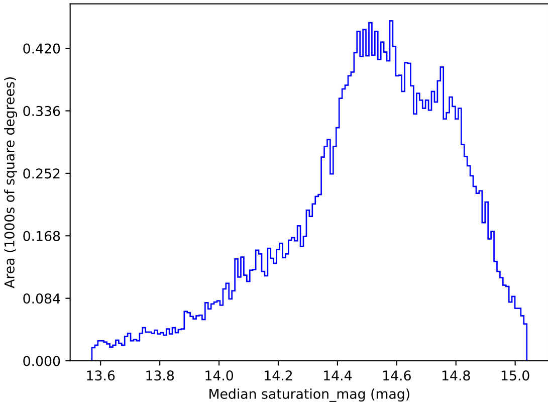
baseline_v3.5_10yrs All sky g band: Median saturation_mag
