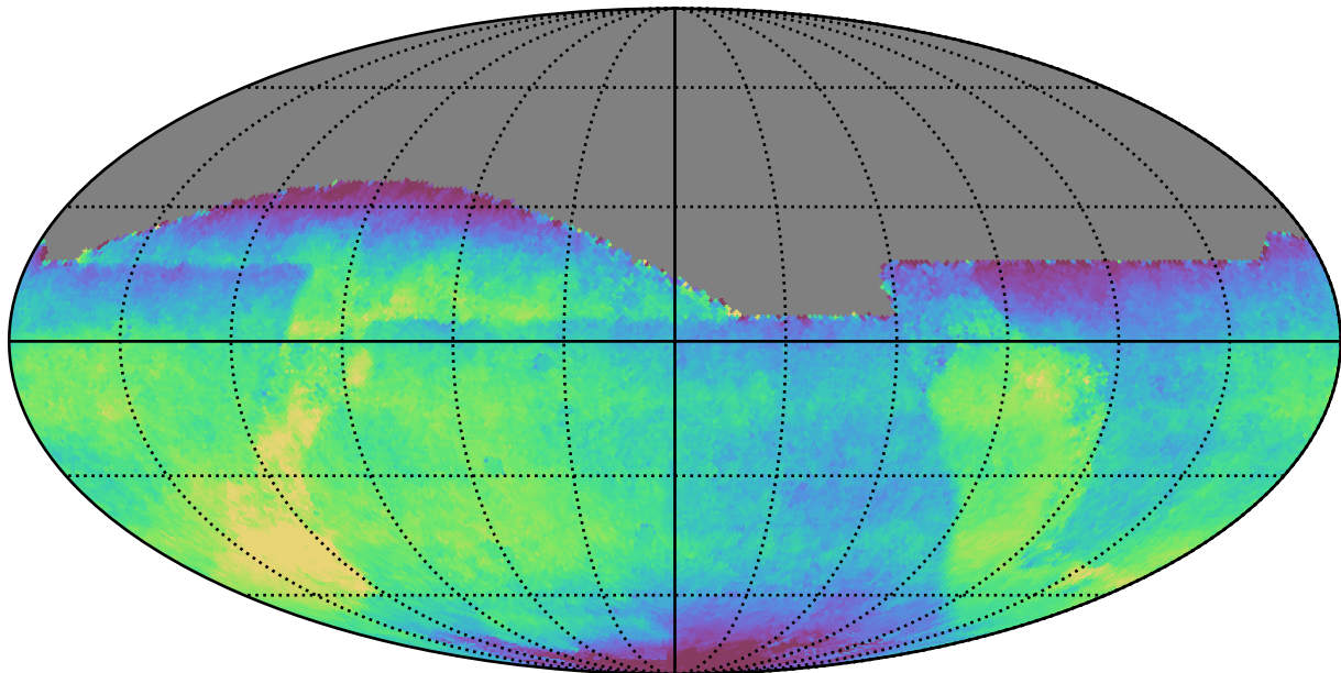
baseline_v3.5_10yrs All sky all bands: Median saturation_mag
