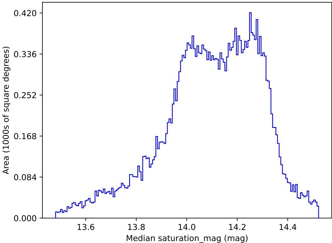
baseline_v3.5_10yrs All sky all bands: Median saturation_mag
