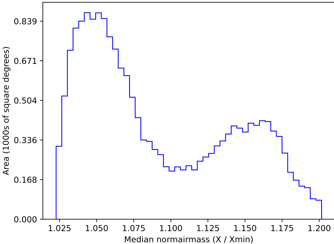
baseline_v3.5_10yrs WFD z band: Median normairmass
