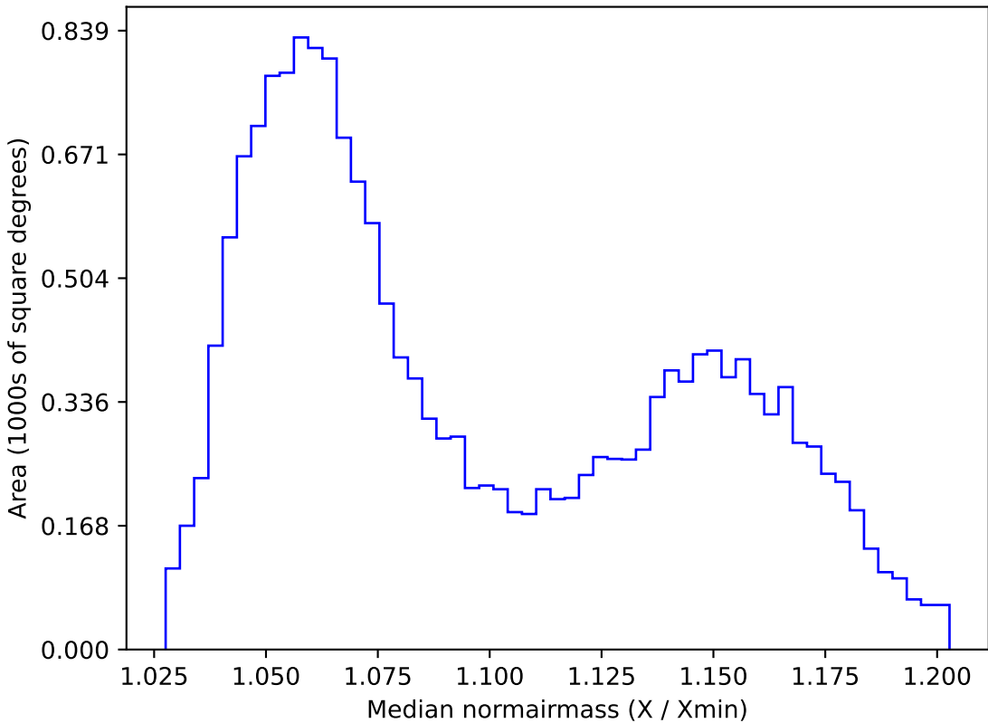
baseline_v3.5_10yrs WFD y band: Median normairmass
