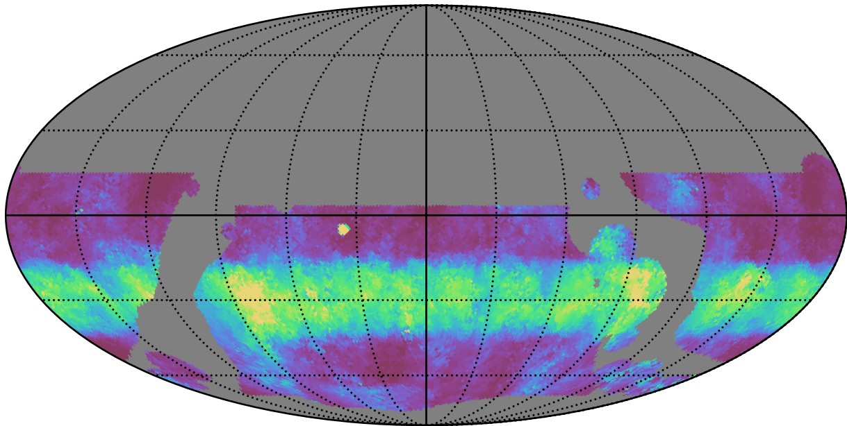
baseline_v3.5_10yrs WFD u band: Median normairmass
