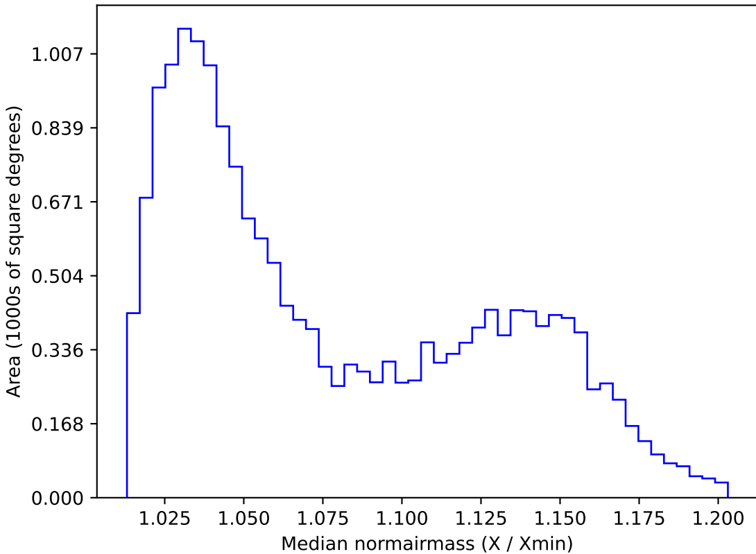
baseline_v3.5_10yrs WFD u band: Median normairmass
