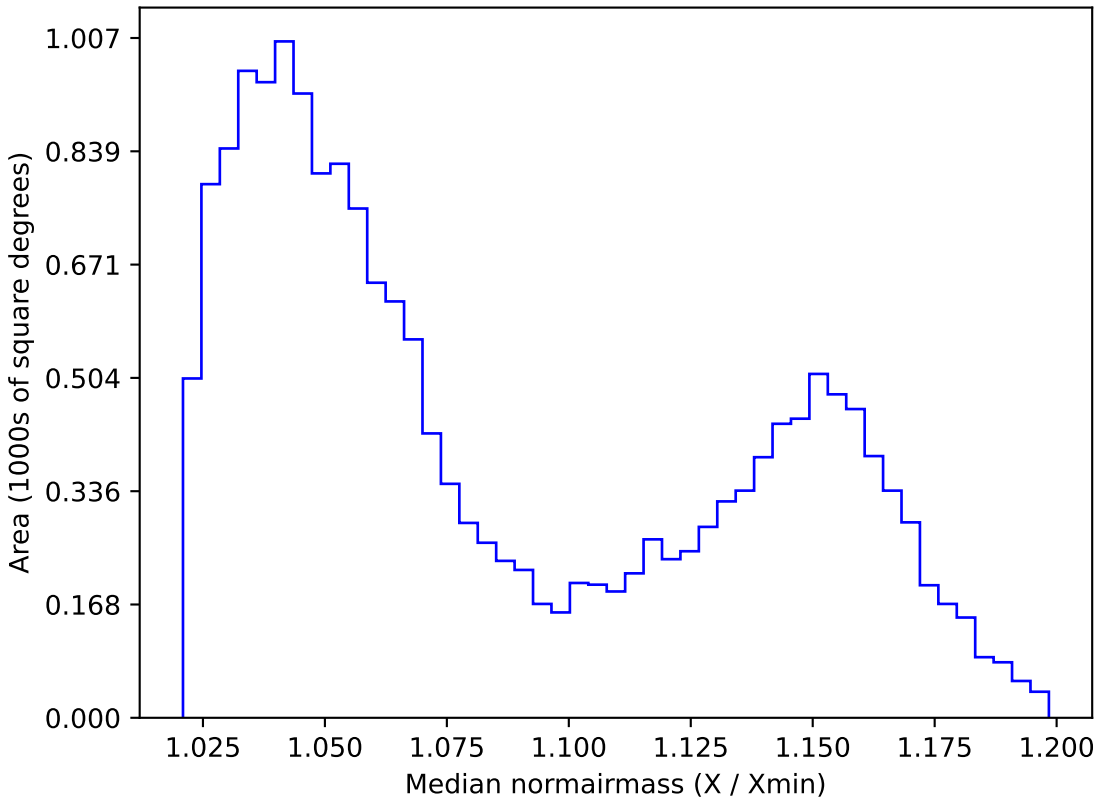
baseline_v3.5_10yrs WFD r band: Median normairmass
