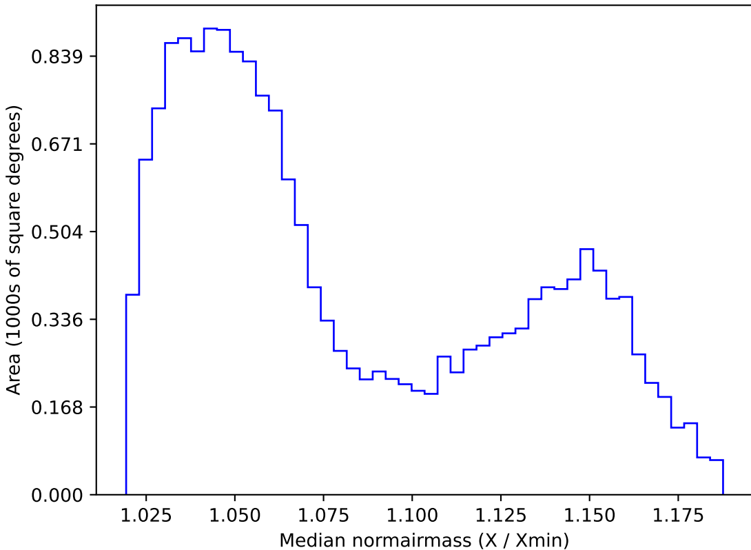
baseline_v3.5_10yrs WFD i band: Median normairmass
