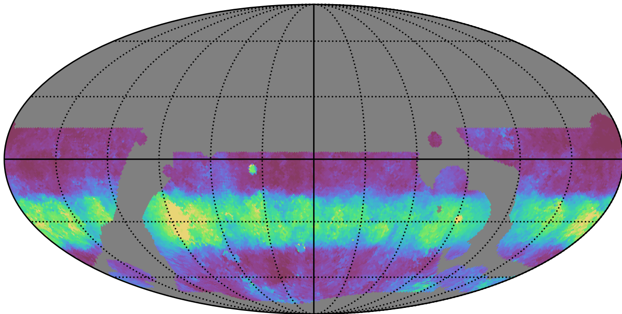
baseline_v3.5_10yrs WFD g band: Median normairmass
