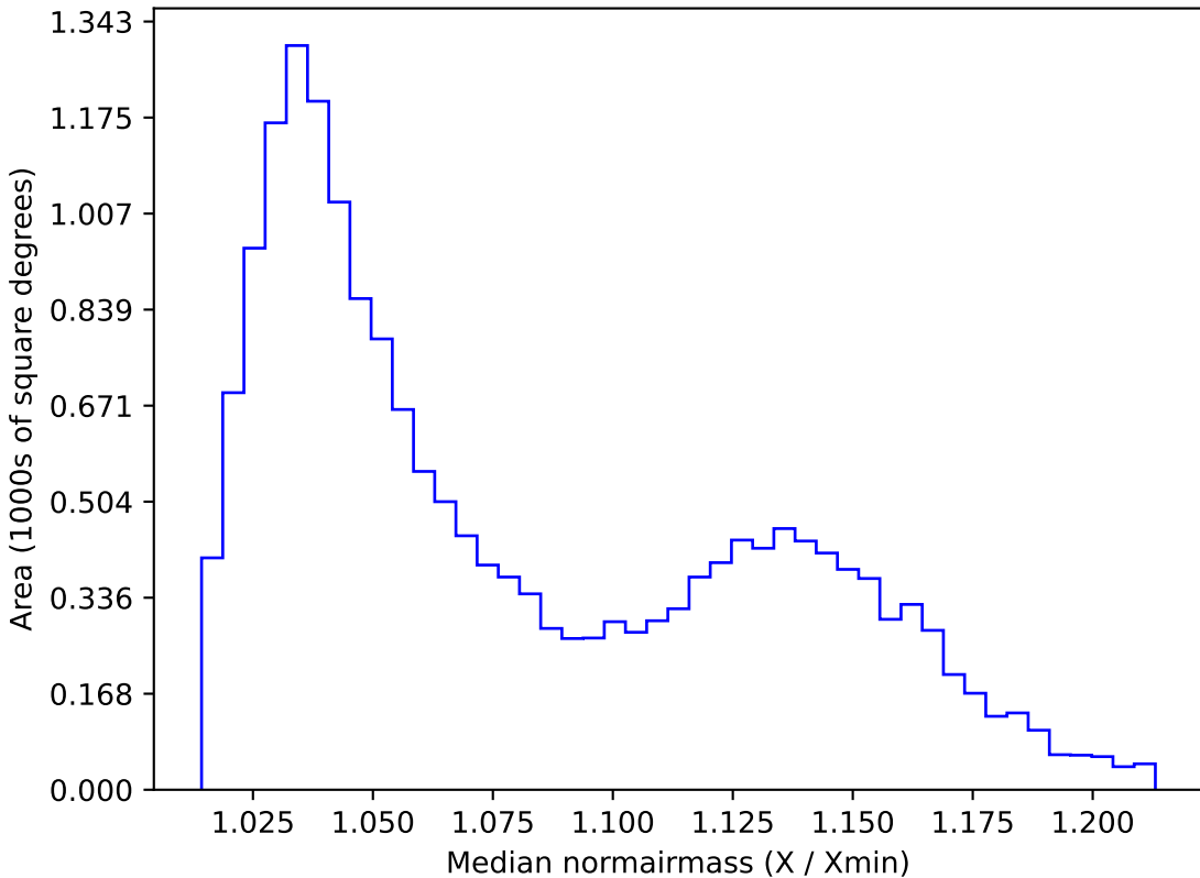
baseline_v3.5_10yrs WFD g band: Median normairmass
