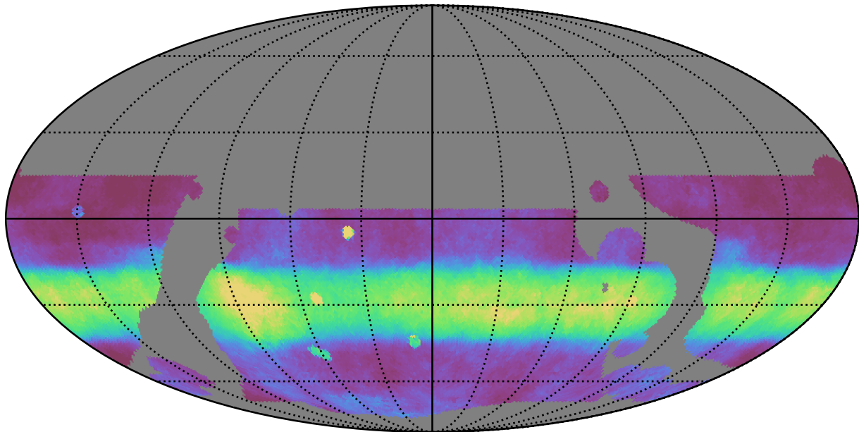
baseline_v3.5_10yrs WFD all bands: Median normairmass
