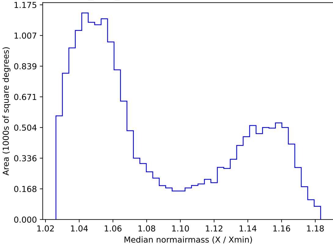
baseline_v3.5_10yrs WFD all bands: Median normairmass
