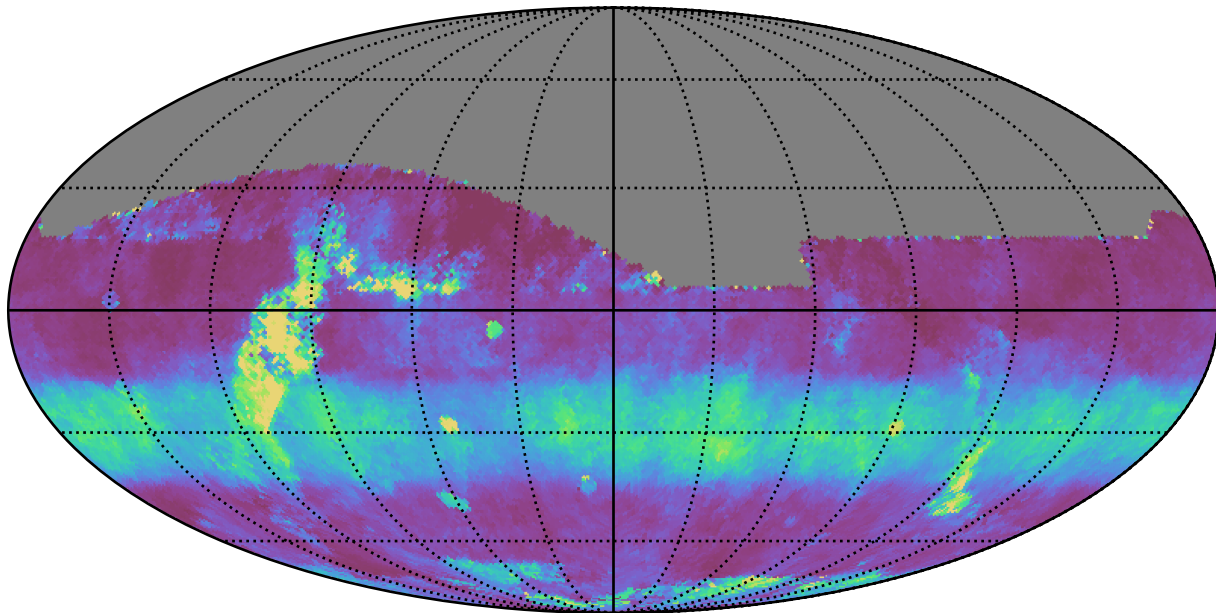
baseline_v3.5_10yrs All sky z band: Median normairmass
