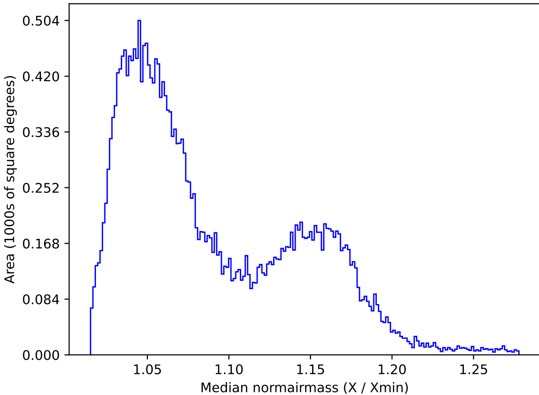
baseline_v3.5_10yrs All sky z band: Median normairmass
