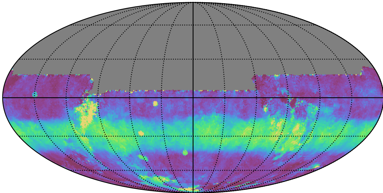
baseline_v3.5_10yrs All sky y band: Median normairmass
