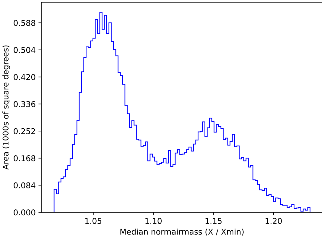
baseline_v3.5_10yrs All sky y band: Median normairmass
