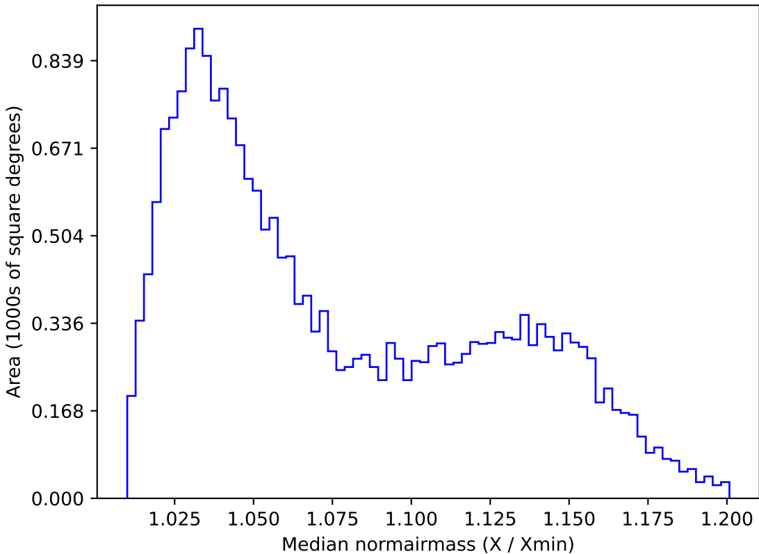
baseline_v3.5_10yrs All sky u band: Median normairmass
