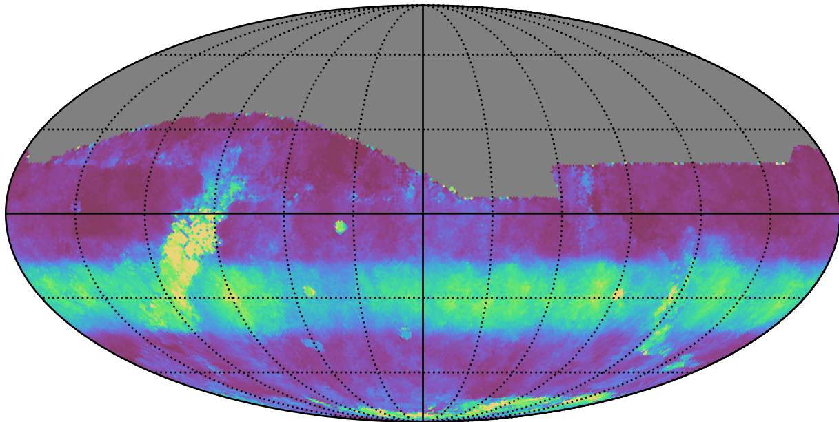
baseline_v3.5_10yrs All sky i band: Median normairmass
