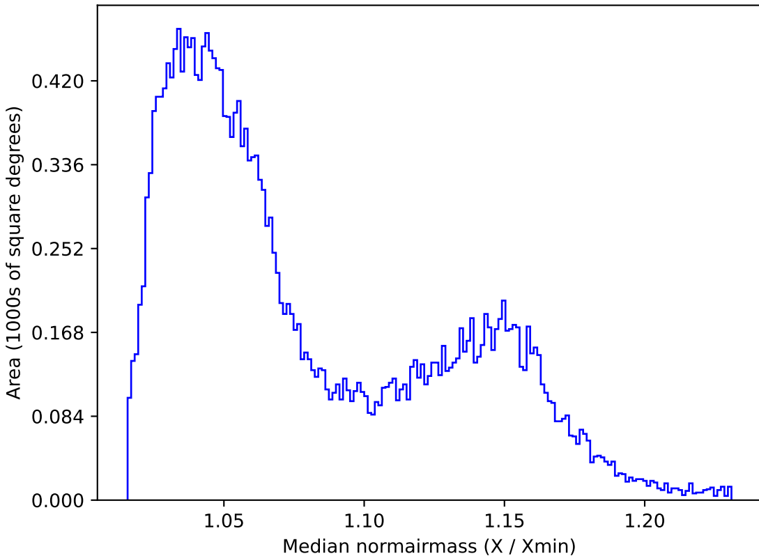
baseline_v3.5_10yrs All sky i band: Median normairmass
