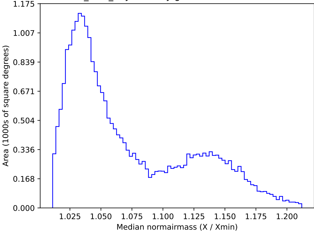
baseline_v3.5_10yrs All sky g band: Median normairmass
