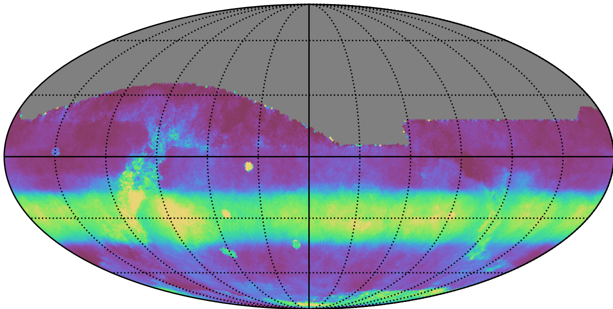
baseline_v3.5_10yrs All sky all bands: Median normairmass
