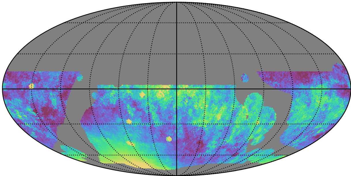
baseline_v3.5_10yrs WFD z band: Median moonDistance
