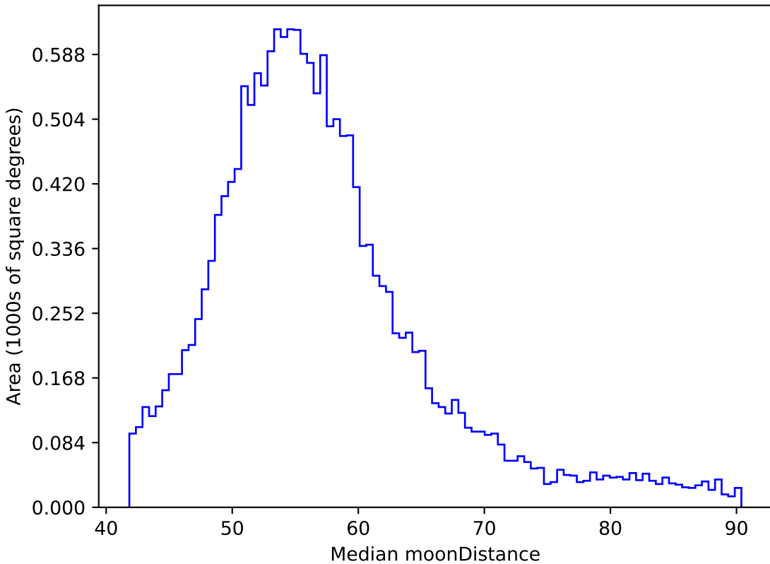
baseline_v3.5_10yrs WFD y band: Median moonDistance
