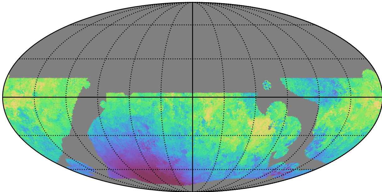
baseline_v3.5_10yrs WFD u band: Median moonDistance
