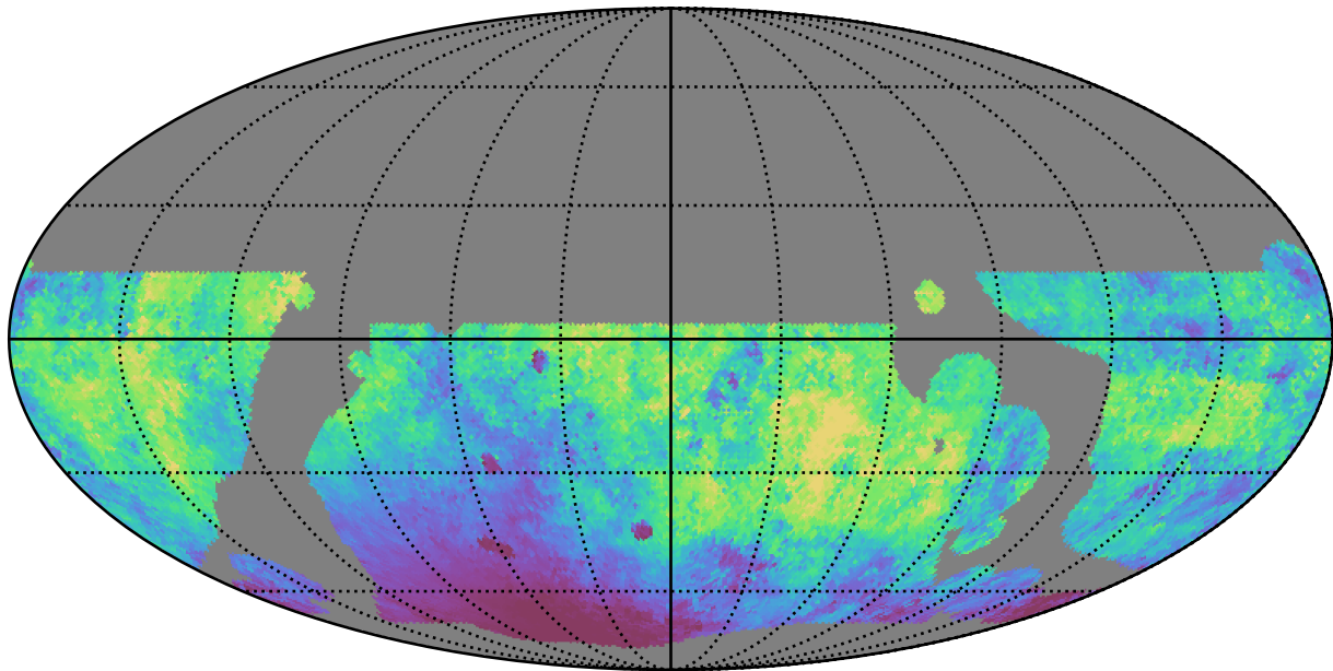
baseline_v3.5_10yrs WFD r band: Median moonDistance
