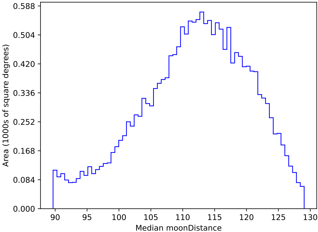
baseline_v3.5_10yrs WFD r band: Median moonDistance
