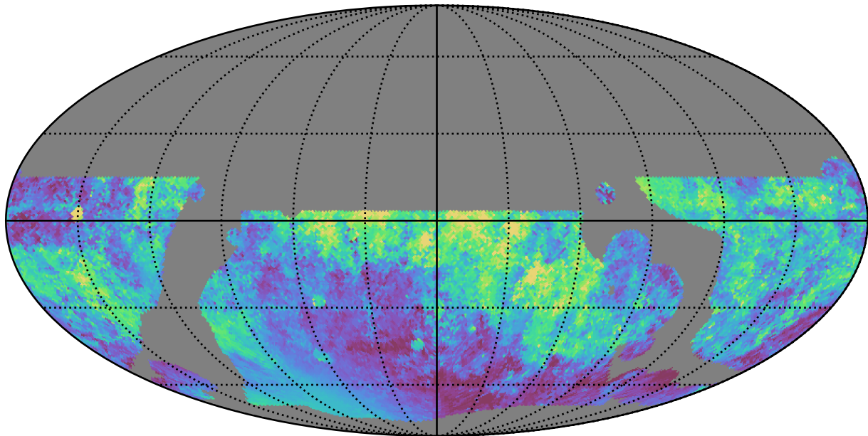
baseline_v3.5_10yrs WFD i band: Median moonDistance
