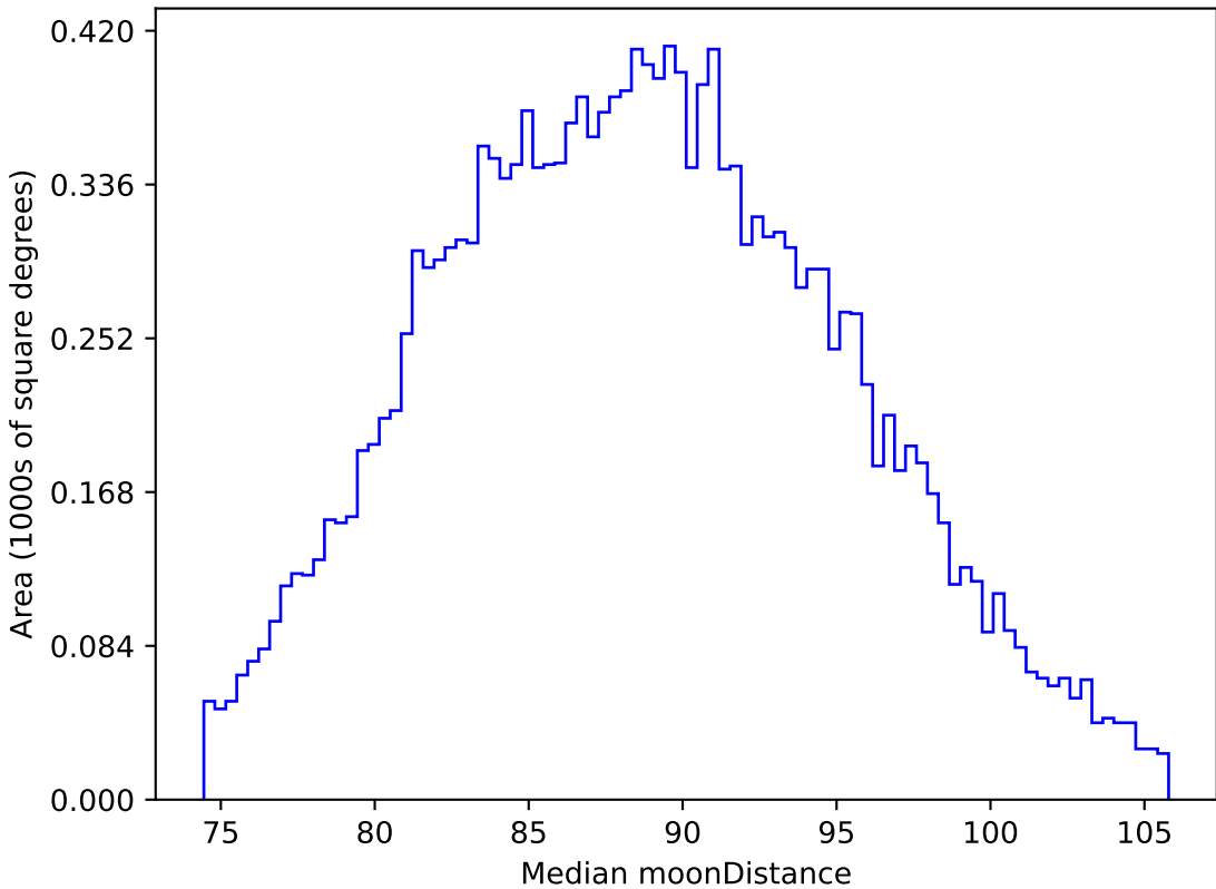
baseline_v3.5_10yrs WFD i band: Median moonDistance
