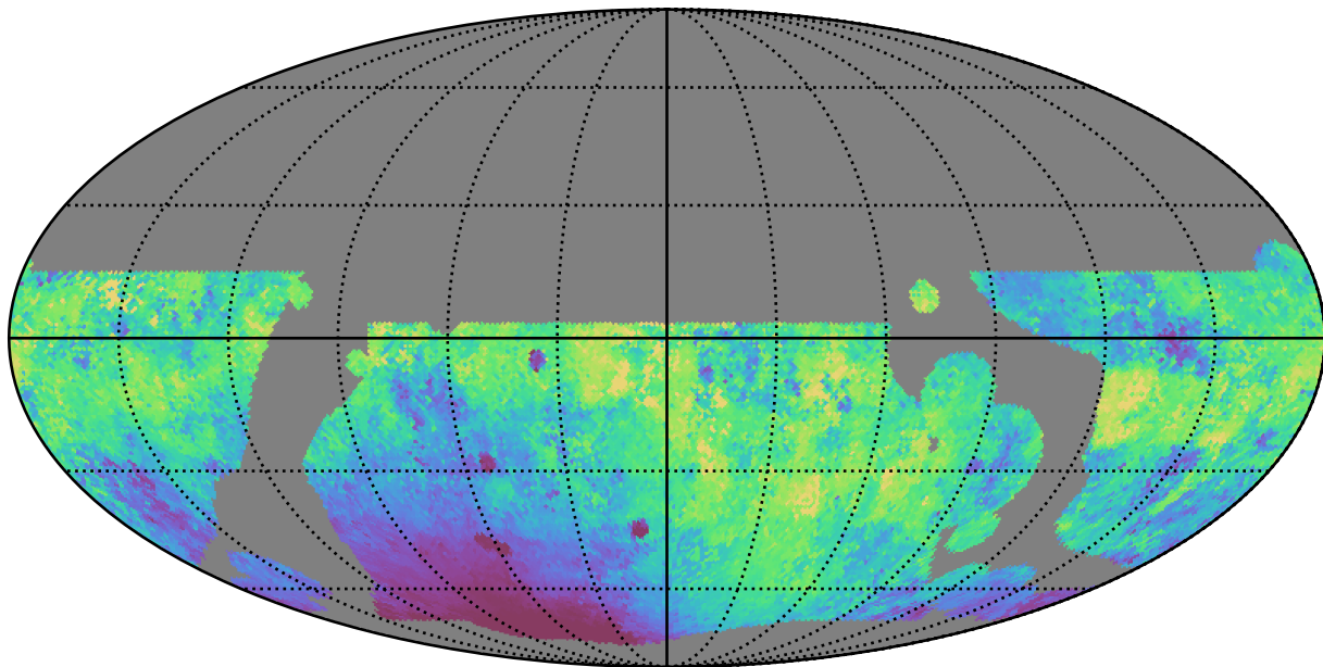
baseline_v3.5_10yrs WFD g band: Median moonDistance
