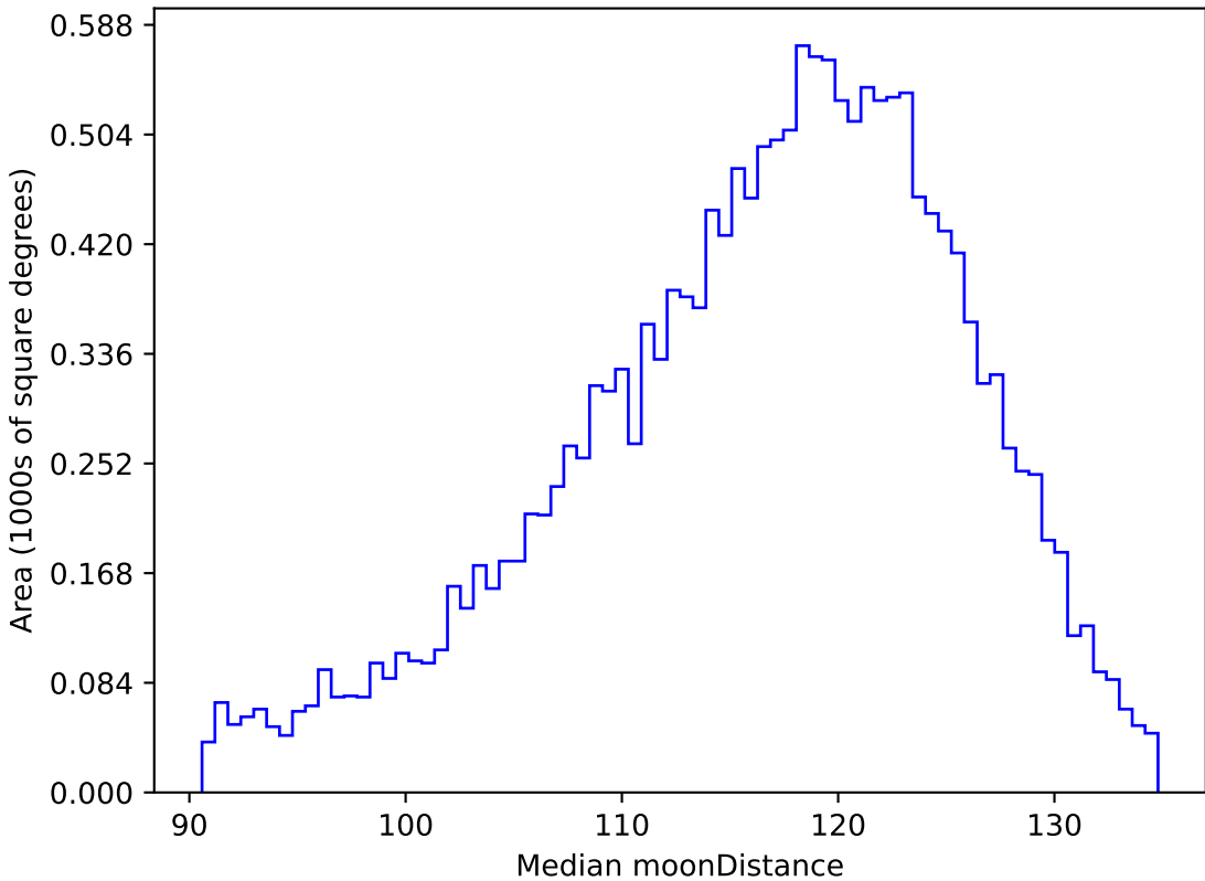
baseline_v3.5_10yrs WFD g band: Median moonDistance
