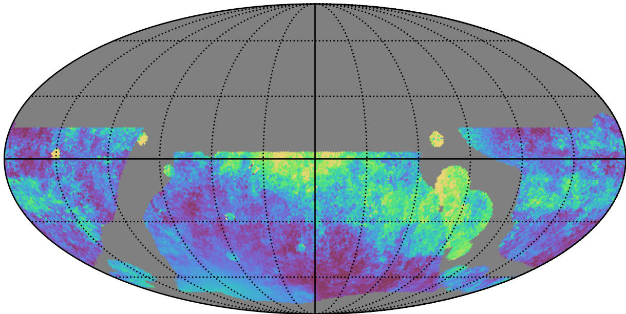
baseline_v3.5_10yrs WFD all bands: Median moonDistance
