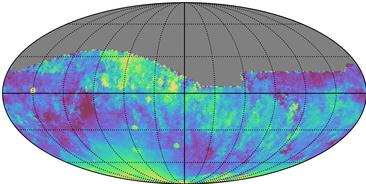
baseline_v3.5_10yrs All sky z band: Median moonDistance
