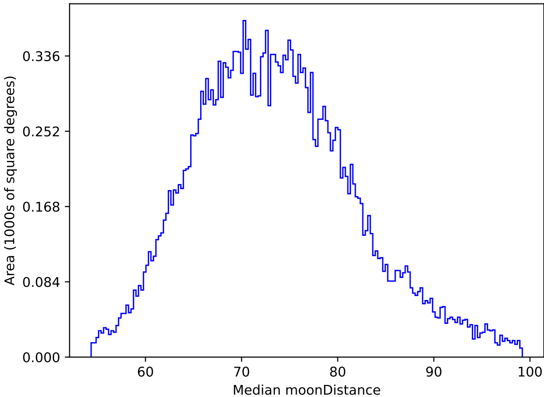
baseline_v3.5_10yrs All sky z band: Median moonDistance
