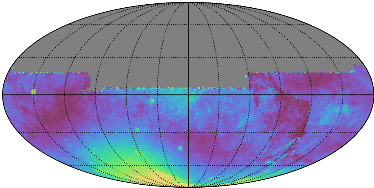
baseline_v3.5_10yrs All sky y band: Median moonDistance
