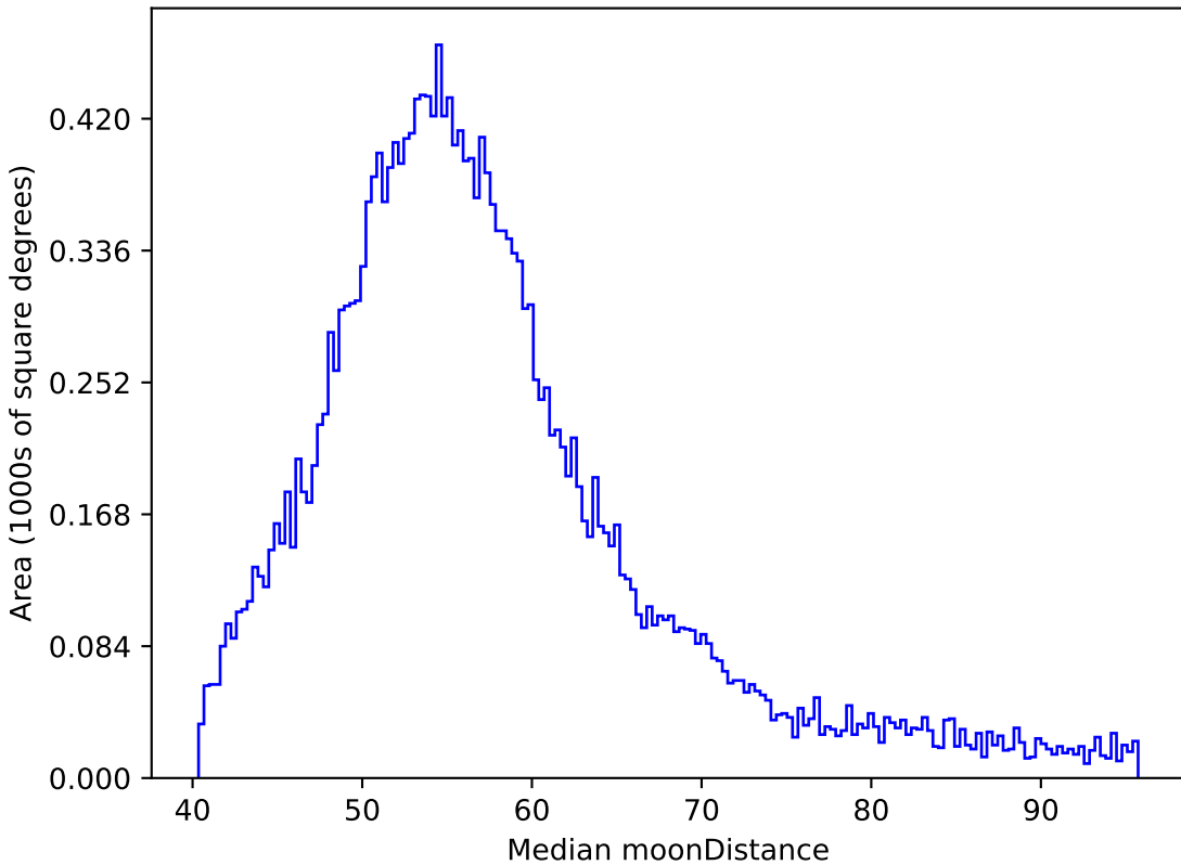
baseline_v3.5_10yrs All sky y band: Median moonDistance
