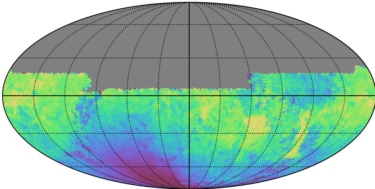
baseline_v3.5_10yrs All sky u band: Median moonDistance
