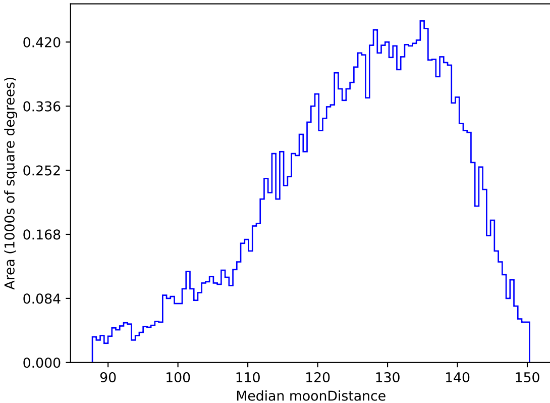
baseline_v3.5_10yrs All sky u band: Median moonDistance
