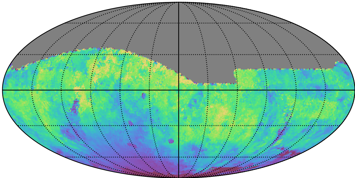
baseline_v3.5_10yrs All sky r band: Median moonDistance
