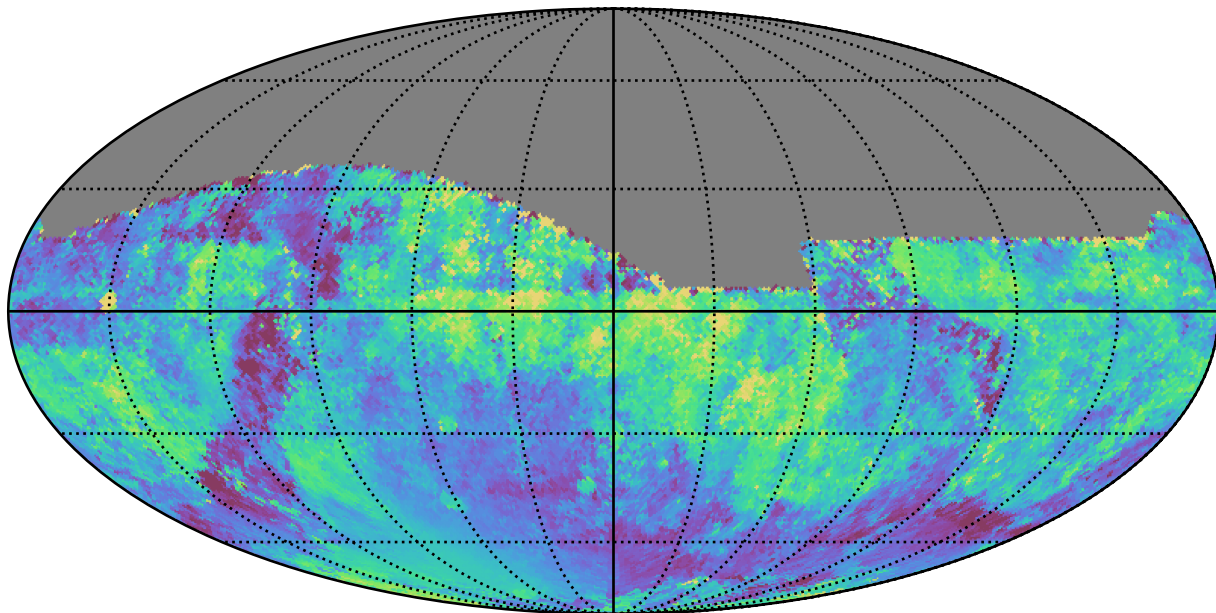
baseline_v3.5_10yrs All sky i band: Median moonDistance
