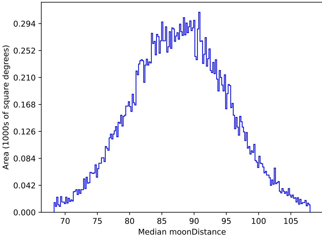
baseline_v3.5_10yrs All sky i band: Median moonDistance
