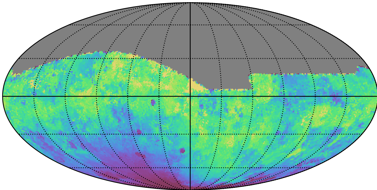
baseline_v3.5_10yrs All sky g band: Median moonDistance
