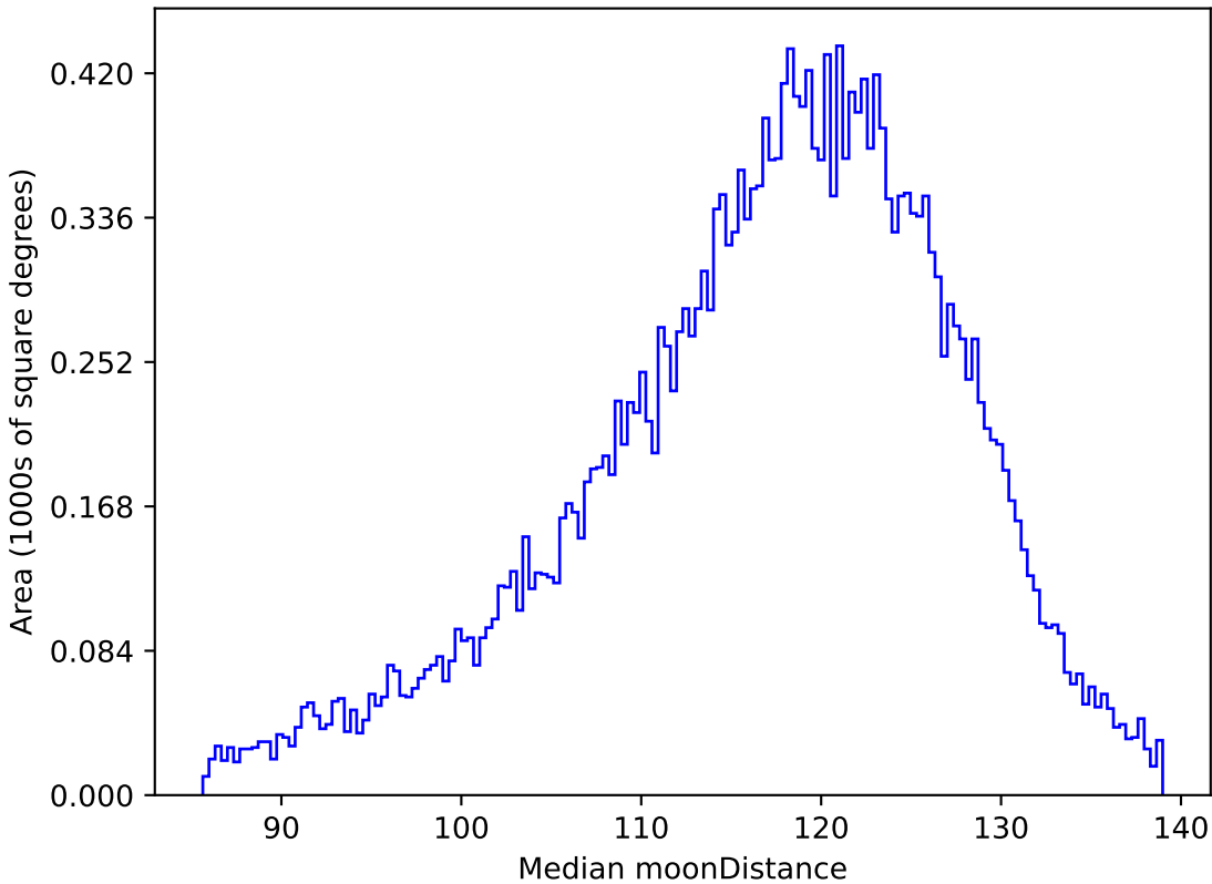
baseline_v3.5_10yrs All sky g band: Median moonDistance
