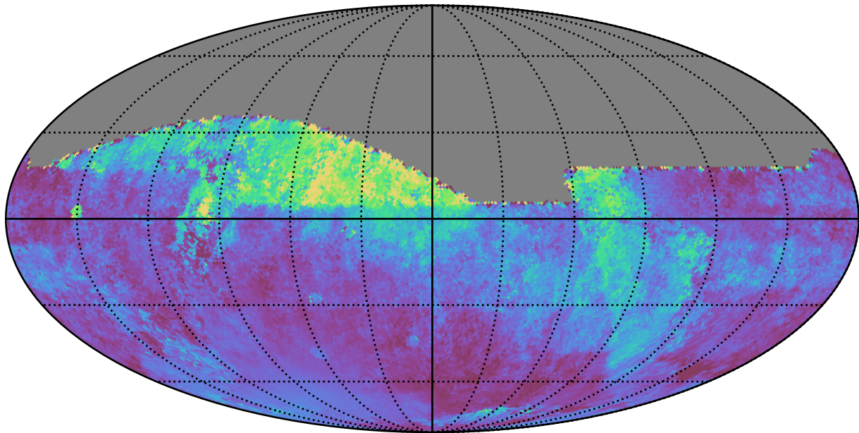
baseline_v3.5_10yrs All sky all bands: Median moonDistance
