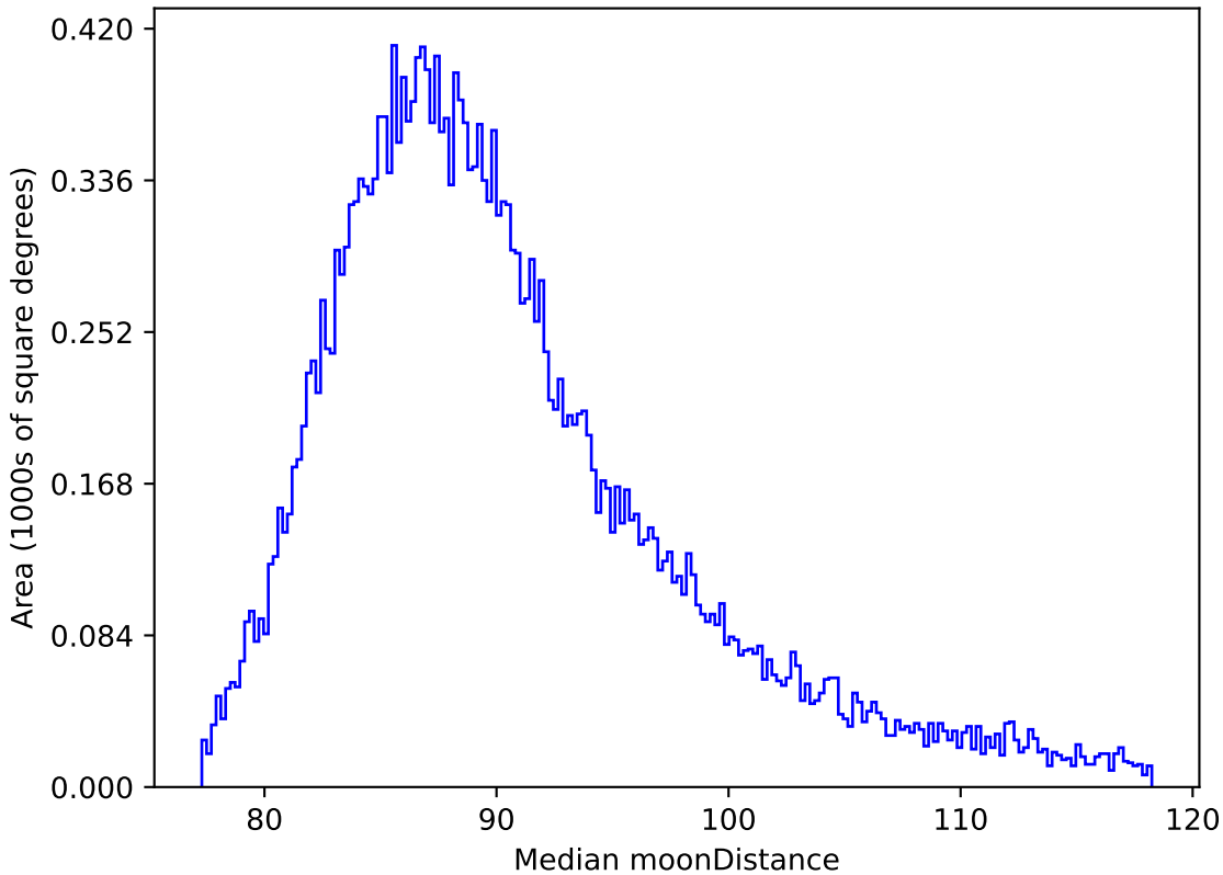
baseline_v3.5_10yrs All sky all bands: Median moonDistance
