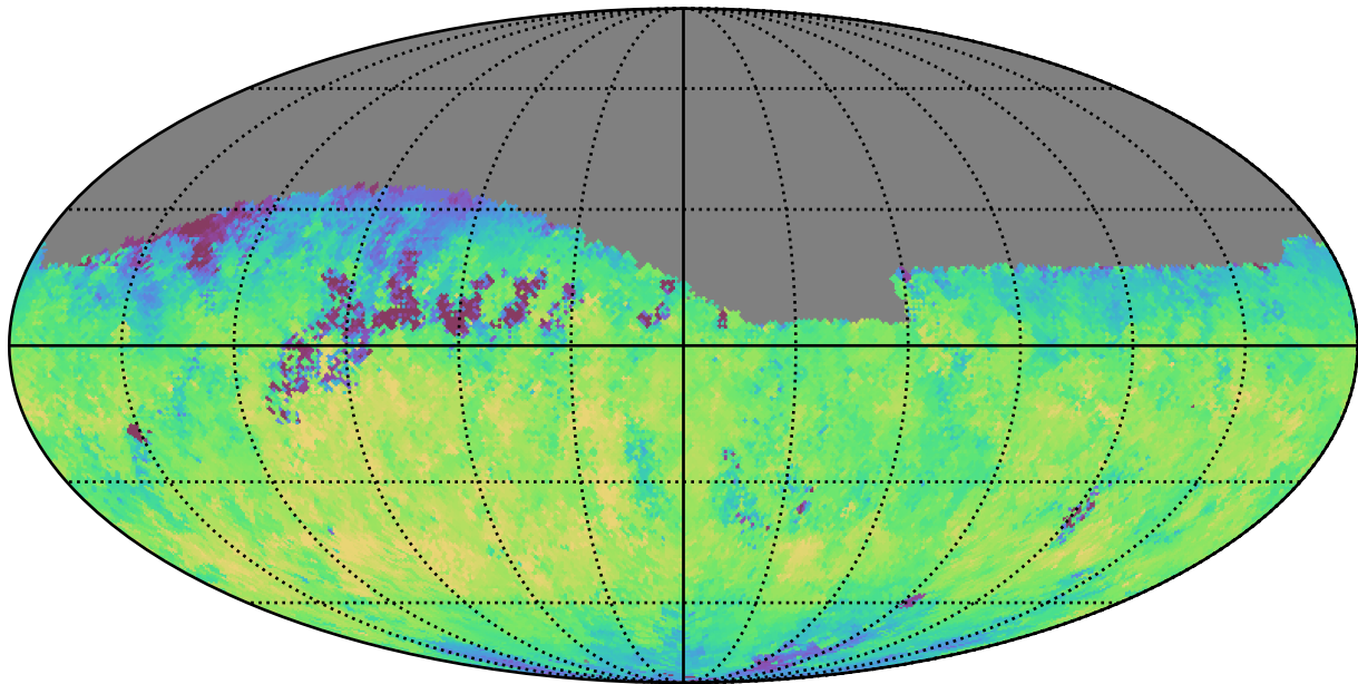
baseline_v3.5_10yrs Yr 1 z band: Median fiveSigmaDepth
