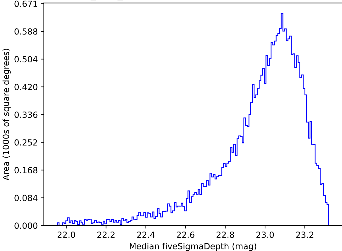
baseline_v3.5_10yrs Yr 1 z band: Median fiveSigmaDepth
