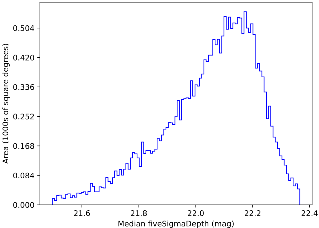
baseline_v3.5_10yrs Yr 1 y band: Median fiveSigmaDepth
