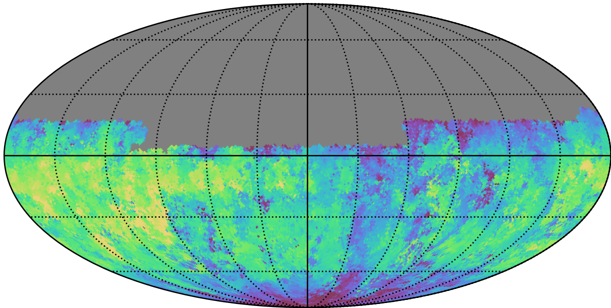
baseline_v3.5_10yrs Yr 1 u band: Median fiveSigmaDepth
