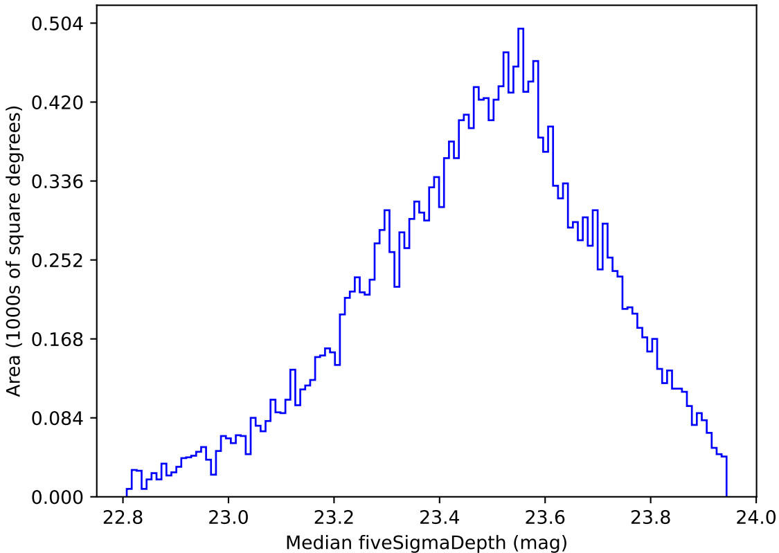
baseline_v3.5_10yrs Yr 1 u band: Median fiveSigmaDepth
